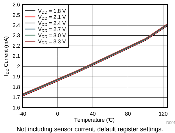
Figure 3. I_{DD} vs Temperature
