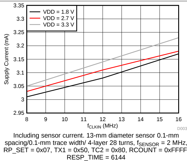
Figure 5. Supply Current (mA) vs f_{CLKIN} (MHz) at 25°C
