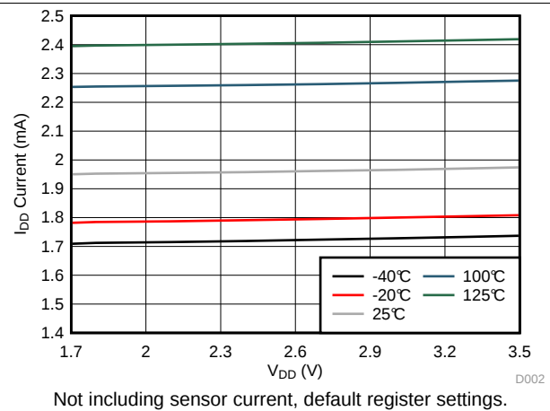
Figure 4. I_{DD} vs V_{DD}
